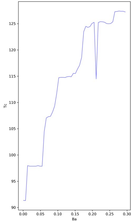
Fig. S9. The virtual sample prediction the highest T_c with Ba by RF model (trained by AFS-1), it also found a dip in the 0.2~0.25 interval of Ba weight, there may be a mysterious physical effect or possible wrong data in the data set.
