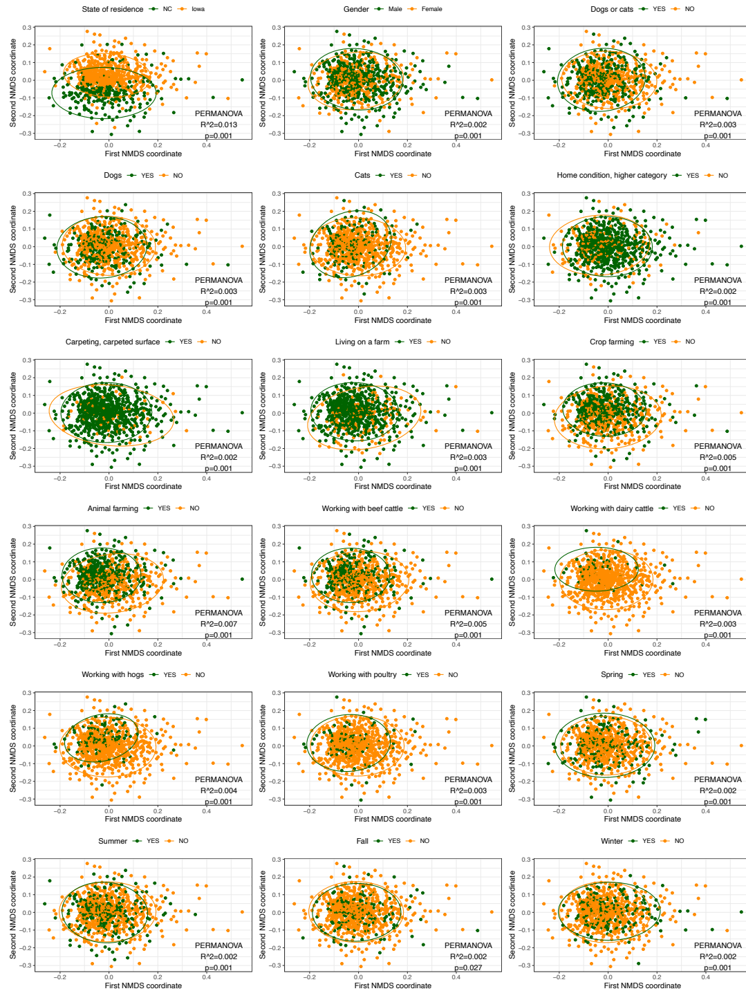
Supplementary Figure S3. Non-metric multidimensional scaling (NMDS) analysis based on unweighted UniFrac distances for all exposures. The dust microbial community of each sample is indicated with one dot. R 2 value (percentage of variance explained by exposure) and p-value from the PERMANOVA analysis are reported.
