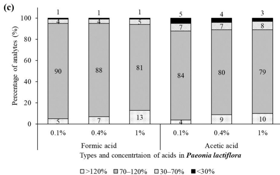
S3 Fig. Distributions of recovery ranges of target pesticides when using 0.1, 0.4, and 1% formic acid or acetic acid in ACN/EA (7:3, v/v).
