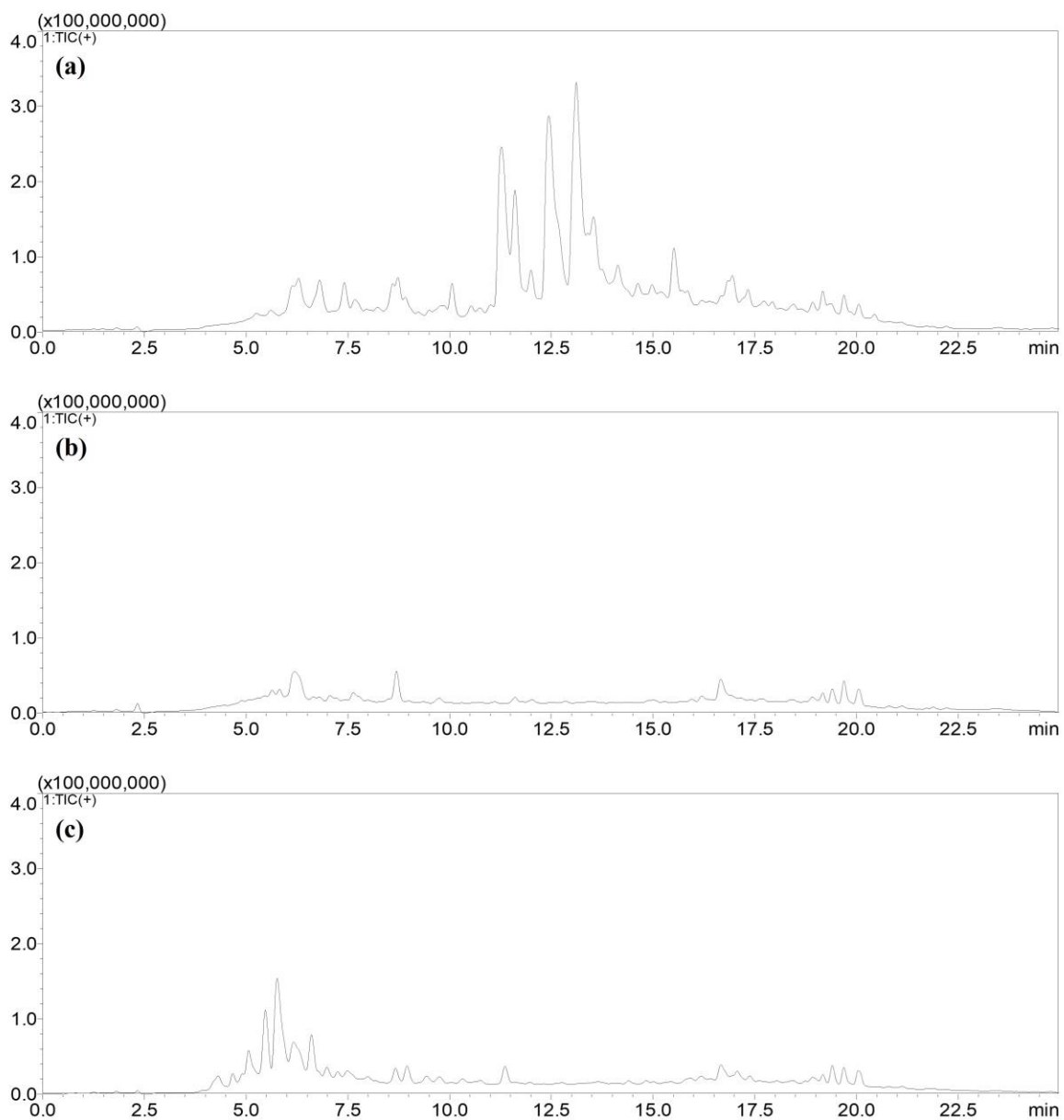
S4 Fig. Total ion chromatograms (TICs) through full scan analysis ( m/z range 50–500). Control (pesticide-free) samples of (a) C. officinale , (b) R. glutinosa , and (c) P. lactiflora were analyzed after preparation using the established method.
