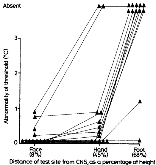
Fig 4 As in fig 3 but for cooling.
