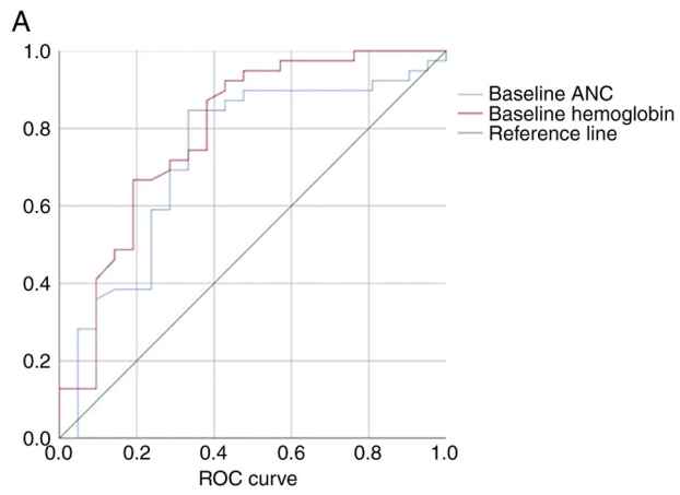
Figure S1. ROC curve analysis of (A) baseline ANC and hemoglobin, (B) baseline IL-6, baseline ferritin and peak ferritin. ROC, receiver operating characteristic; ANC, absolute neutrophil count.
