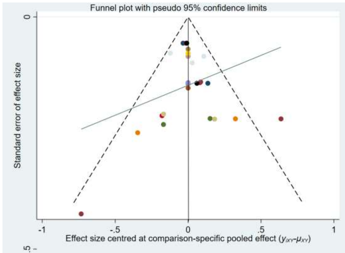
Figure S3. Funnel plots.
