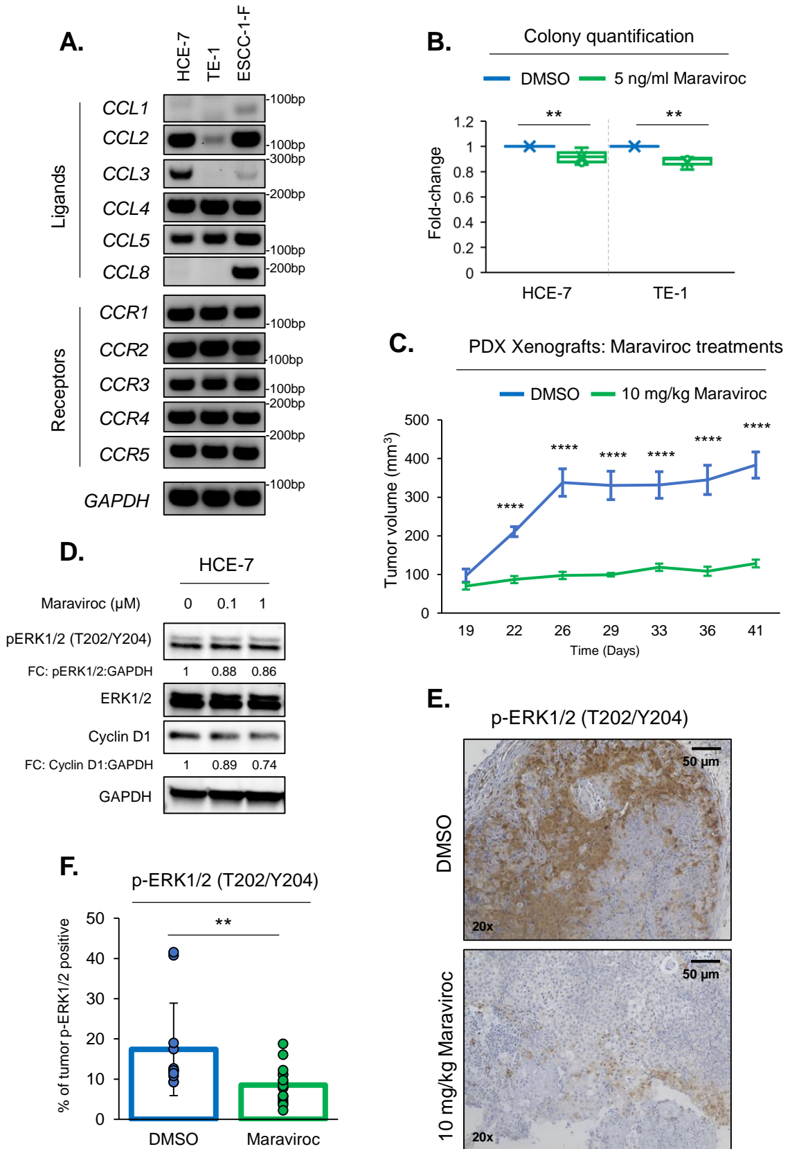
Fig. S4: Targeted CCR5 inhibition replicates CCL5 loss with reduced tumor cell proliferation in vitro and in vivo
