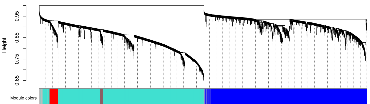
Cluster Dendrogram
