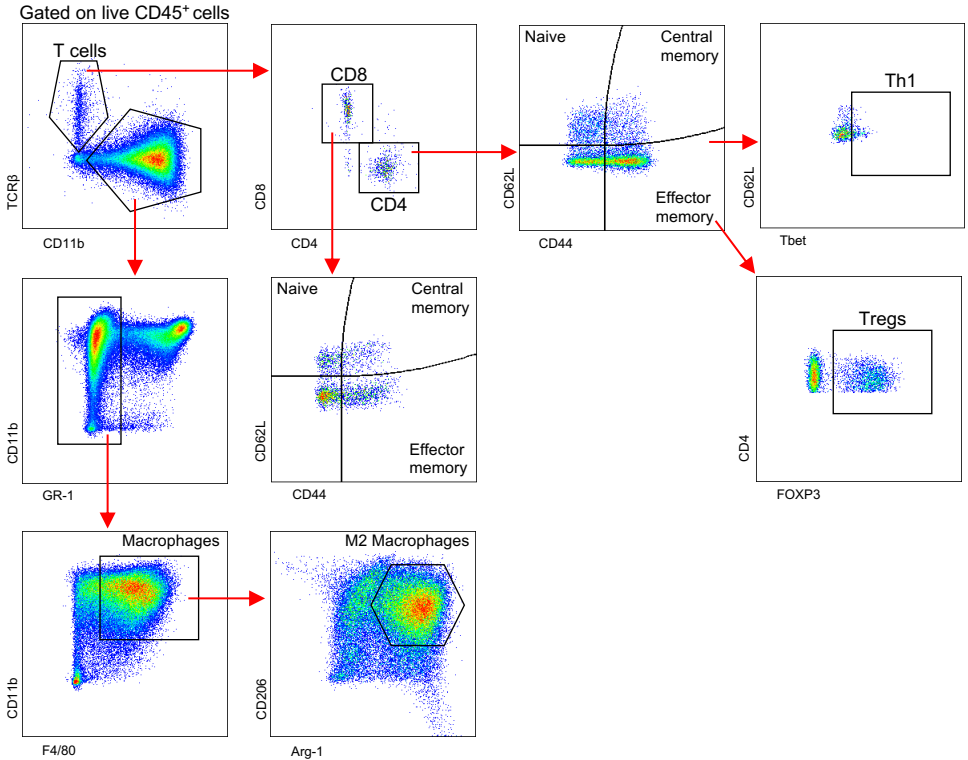
Supplementary Figure S3. Gating strategies used for flow cytometry analysis. Representative dot plots depict gating strategies used for intratumoral macrophages and T-cell analysis in flow cytometry experiments in PKT mice across all treatment cohorts.
