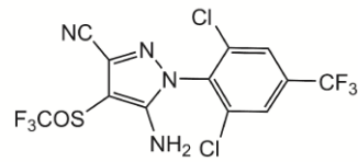
1988 Fipronil phenylpyrazole
