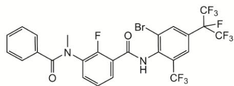
2013 Broflanilide meta-diamide
