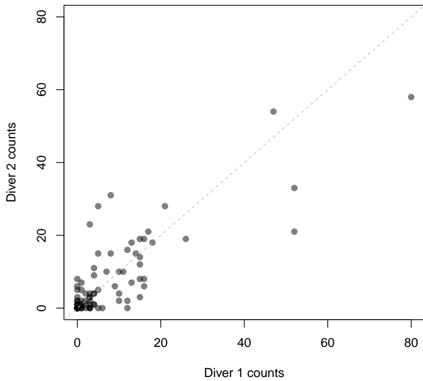
Figure S1: Counts from Diver 1 and Diver 2 on repeated quadrats in 11 transects from Little Birch Lake. The dotted line represents the ideal case where no observational error is present in the counts.
