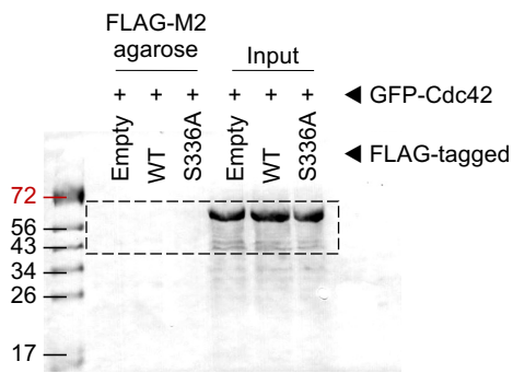
Fig 6b. Ponceau
