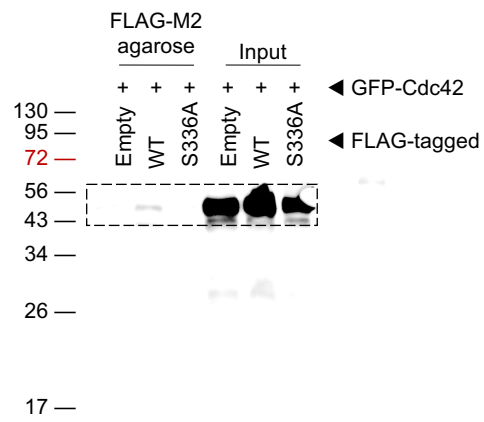
Fig 6b. GFP
