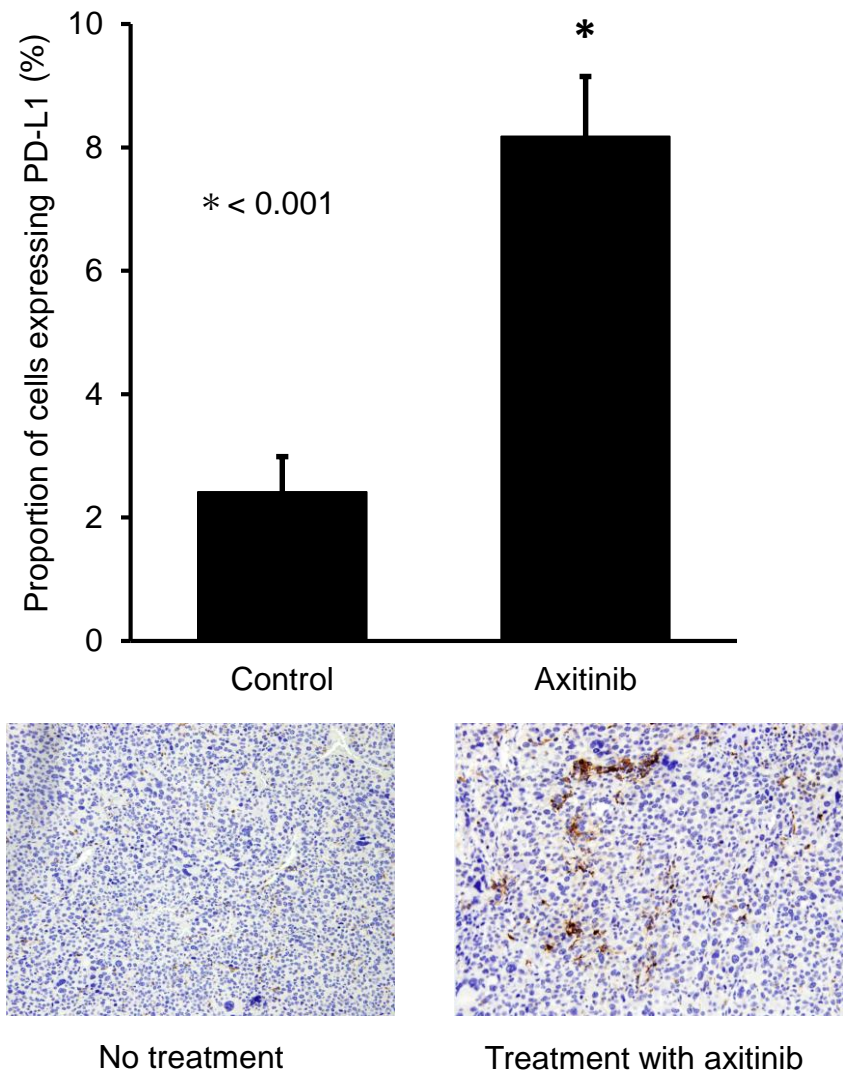
Supplementary Figure 2 :Proportion of cells expressing PD-L1 / PD-L2 in vivo
