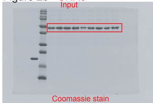
Figure 2b SNX1
