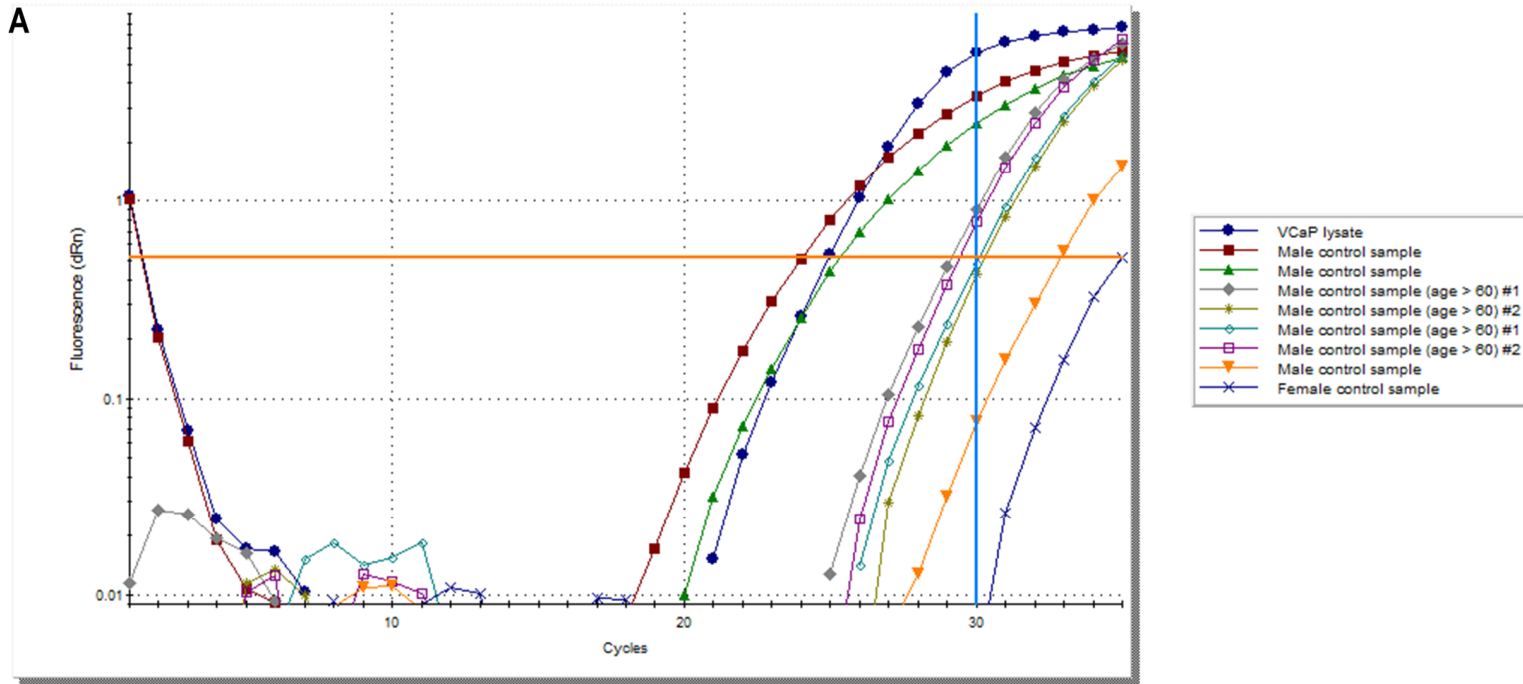
Amplification Plots, mRNA ERG
