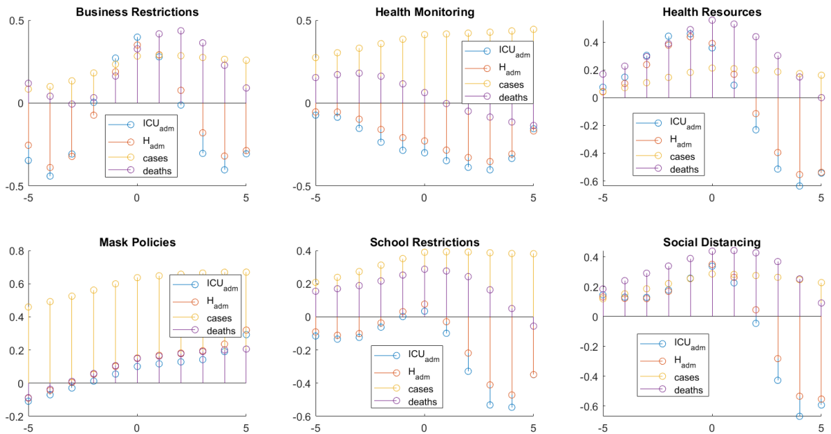
Figure 1. Cross-correlation between indices and epidemiological variables for France. x lag value, y cross-correlation value
