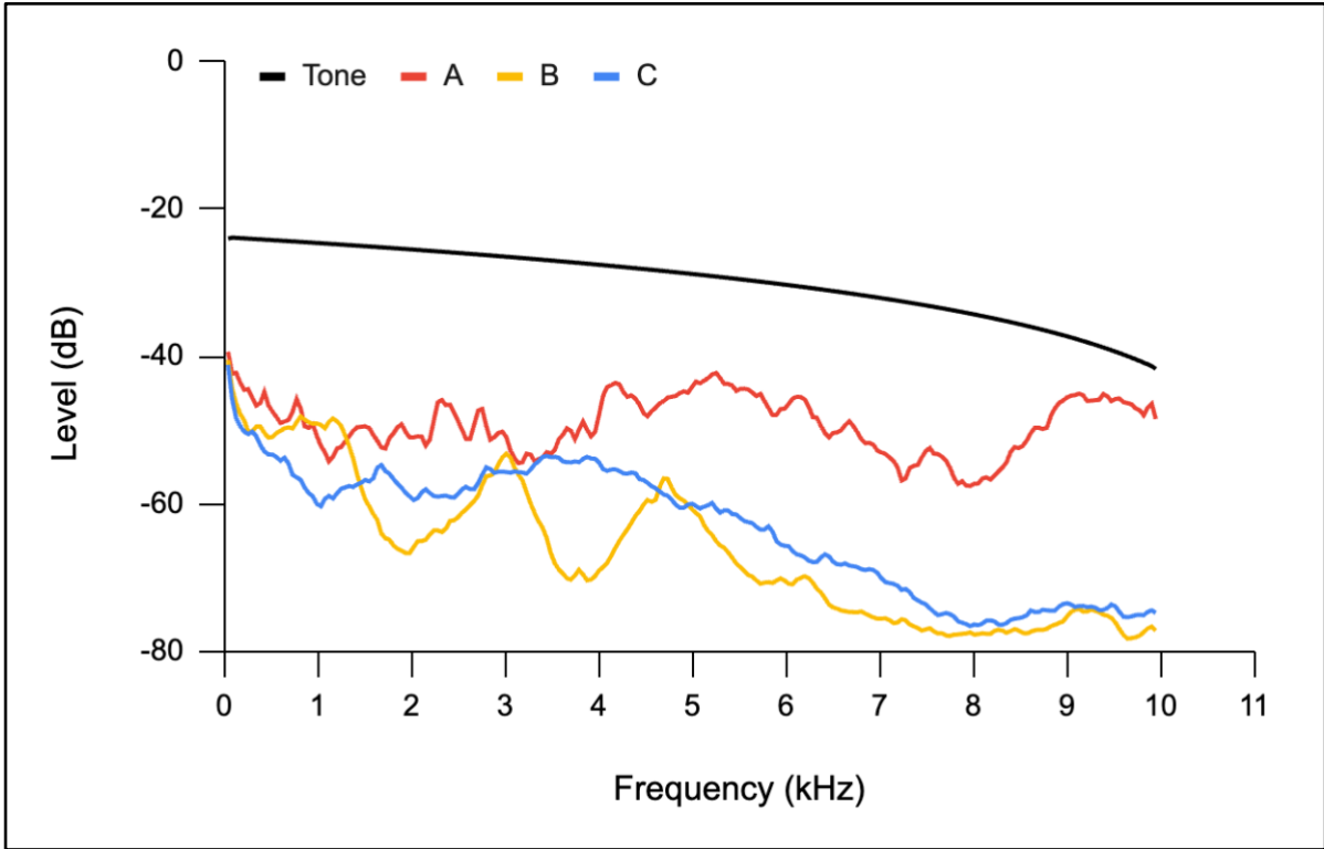
S1 Fig. The frequency response of recorders A, B, and C with respect to the generated tone (black line) in Audacity® [40]. The spectrum was computed using a default 1024-point FFT analysis. The frequency range is 0-10 kHz.
