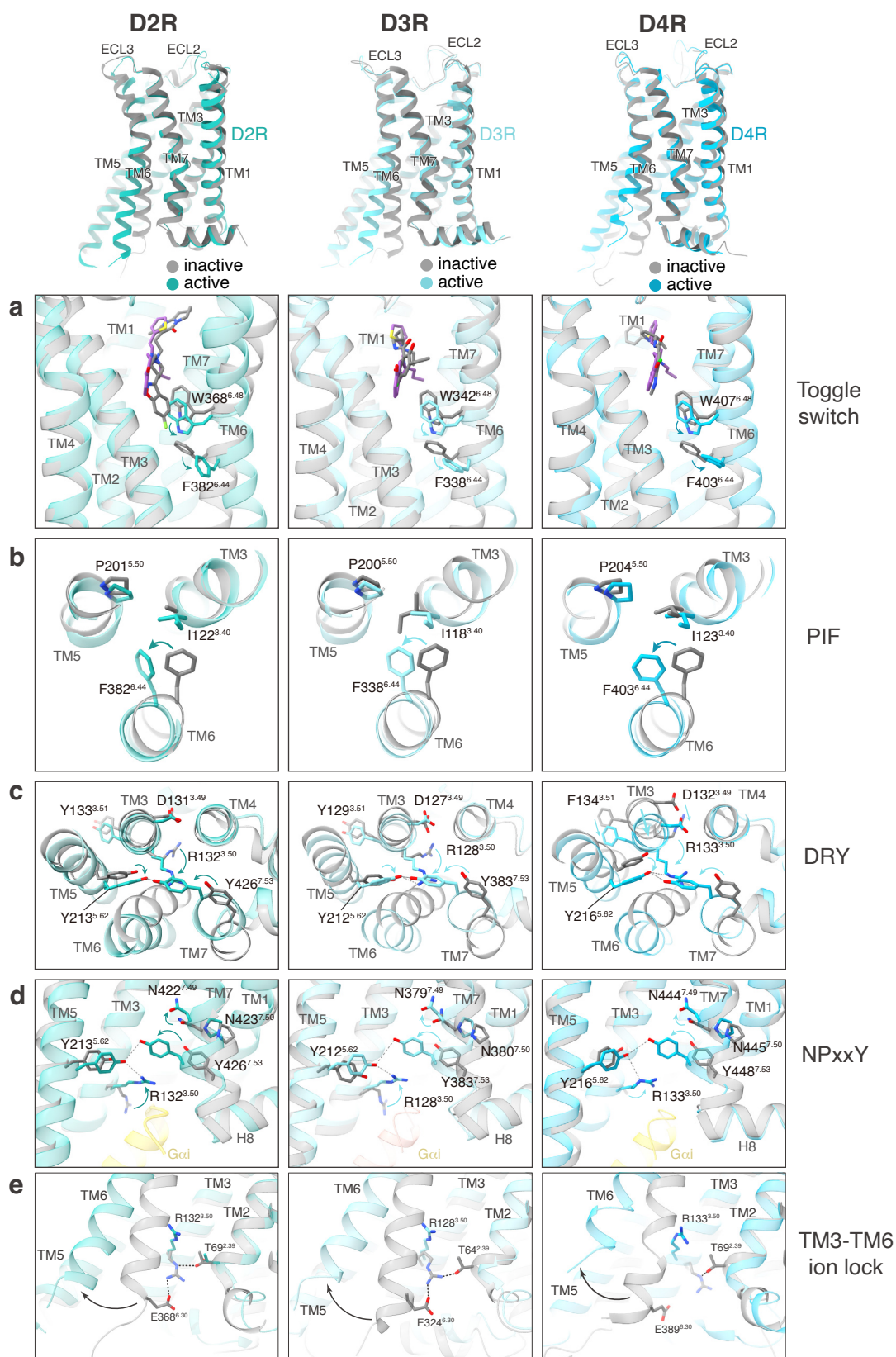
Fig. S6. D2-like receptors activation. a Toggle switch induced by agonist binding in D2R, D3R, and D4R. b Conformational change of PIF motif in D2R, D3R, and D4R. c Conformational change of DRY motif in D2R, D3R, and D4R. d Rotation of the NPxxY motif in D2R, D3R, and D4R. e The breaking of TM3-TM6 ion lock of D2R, D3R, and D4R.
