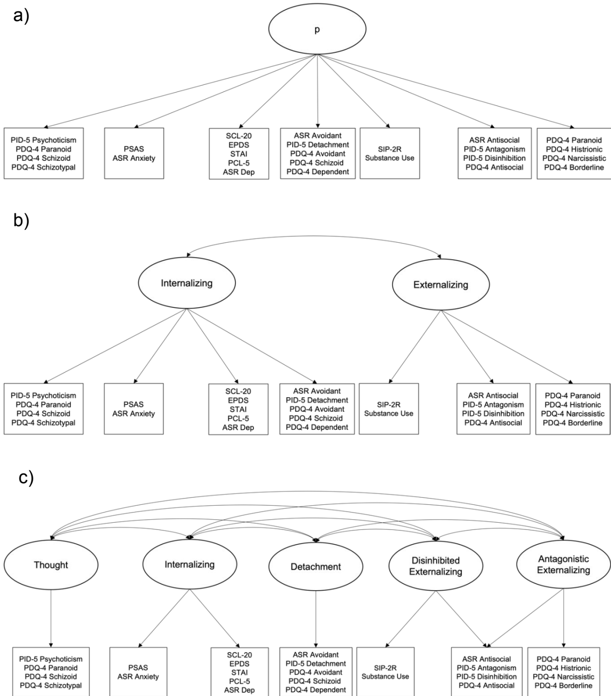
Figure S1. Unidimensional model of psychopathology (a); correlated two-factor model of psychopathology (b); correlated five-factor model of psychopathology (c).
