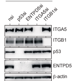
j OC58 (OVCA) p53 R175H
