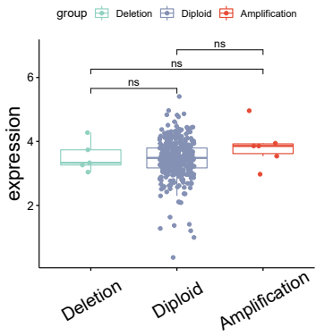
F NSUN5_ANOVA_tests:p=0.249
