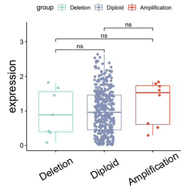
G NSUN7_ANOVA_tests:p=0.579
