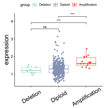
D NSUN3_ANOVA_tests:p=3.151e-04
