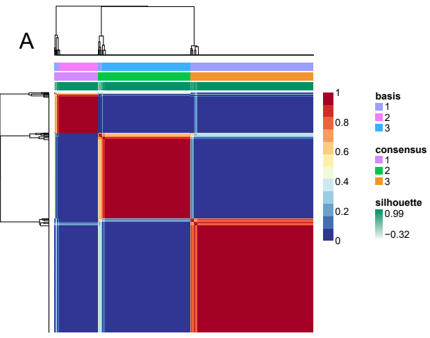
Consensus matrix
