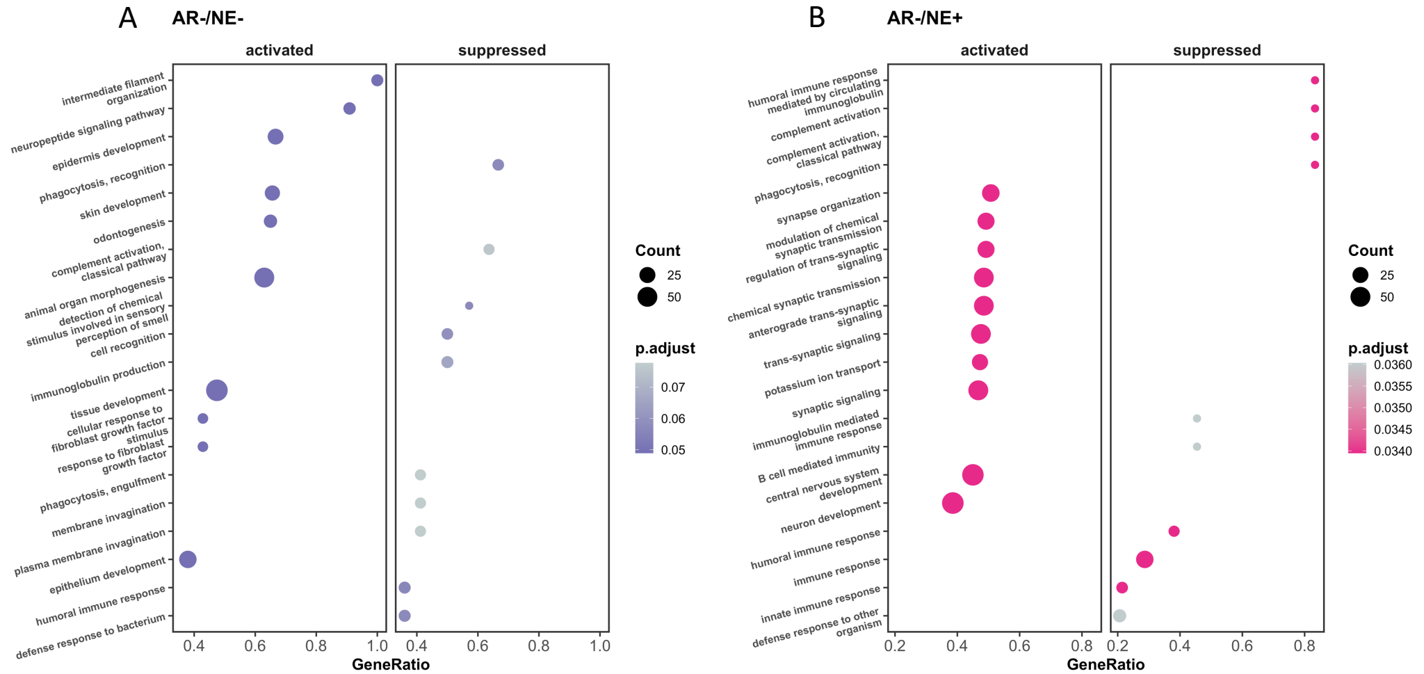
Supplementary Figure 4. Gene Ontology (GO) with Biological processes (BP) on the genes uniquely up- or down-regulated within each subtype.
