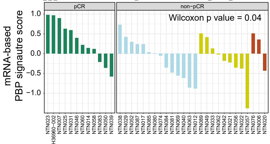
Supplementary Figure 3. Bar plot shows the levels of the PBP signature score in pCR samples (RCB 0) and non-pCR samples (RCB I/II/III) measured by the KIPA (A), the proteomics (B), and the RNA-seq (C). P-values were determined by the Wilcoxon rank-sum test comparing signature levels for pCR samples to non-pCR samples.
