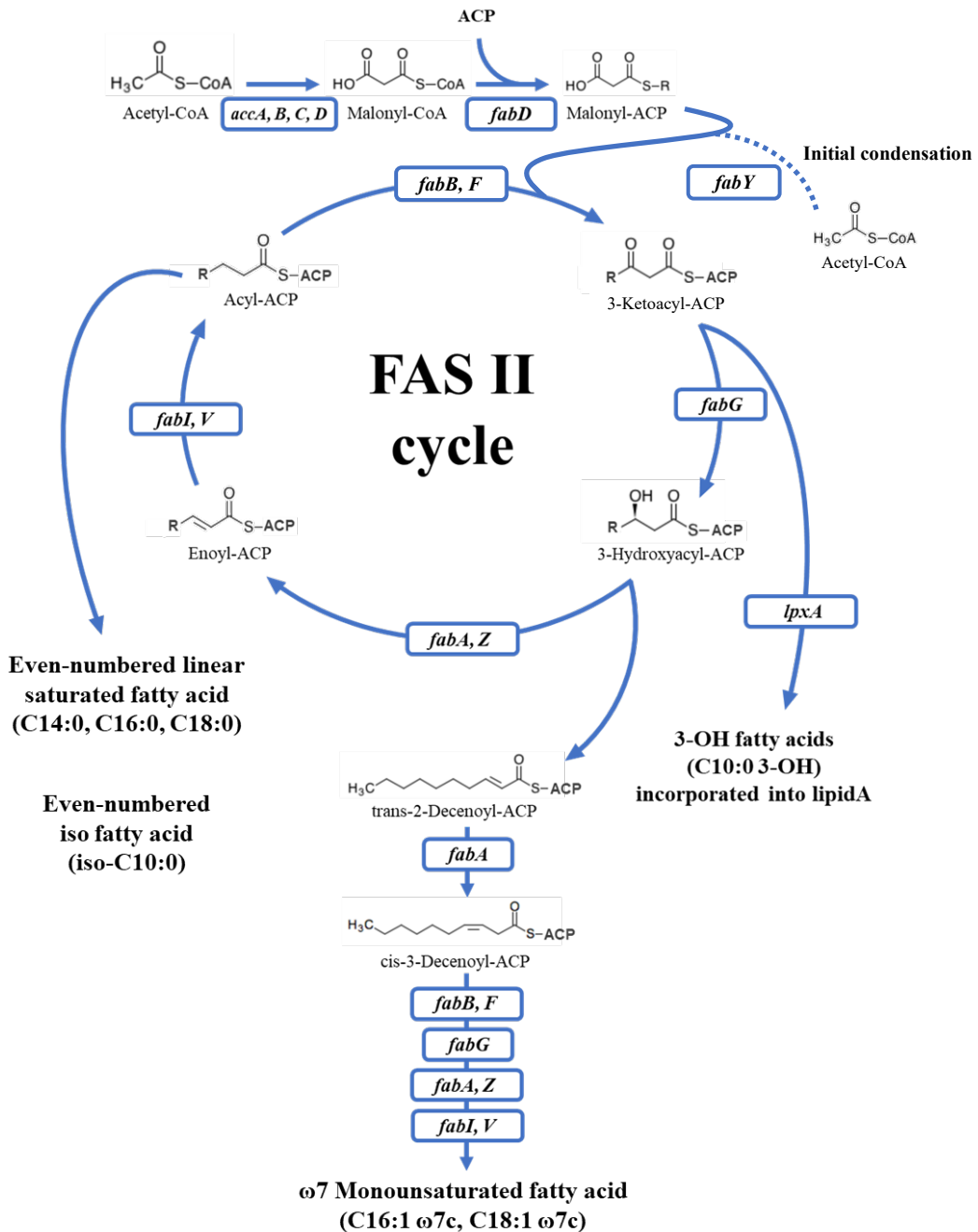
S4 Fig. Predicted fatty acid synthetic pathway in Neptuniibacter .
