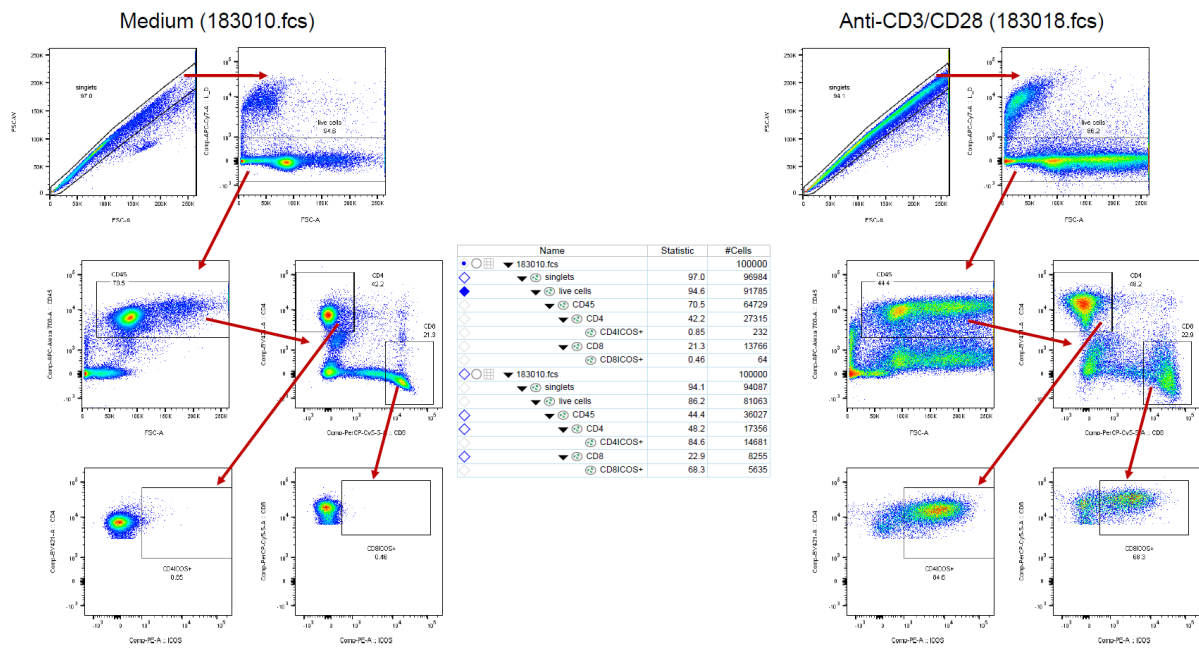
Supplementary Fig. 1. Exemplar flow cytometry gating strategy. Associated with Fig. 1a, Fig. 2a, e, f, Fig. 3c, e, f, Supplementary Fig. 6f and Supplementary Fig. 10f. Example shown for ICOS.
