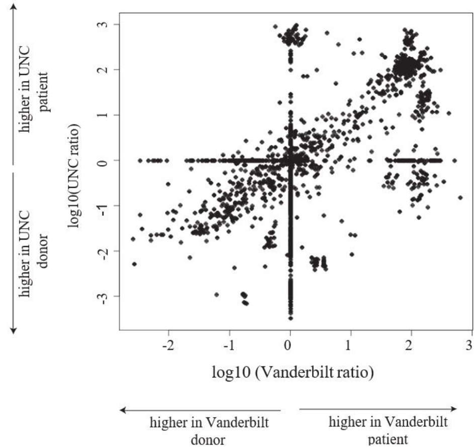
Supplemental Figure 2. For each gene from HumanN (see supplementary Table 1), the \log_{10} of the ratio of the average of all timepoints for each patient divided by the corresponding value for the donor. The x-axis show this ratio for the Vanderbilt patient and the y-axis show this ratio for the Chapel Hill patient.
