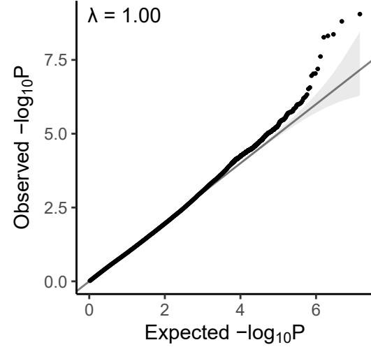
mChrY-loss
