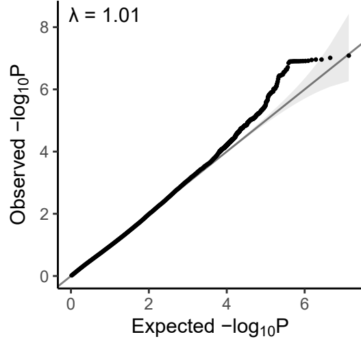
ChrX Loss
