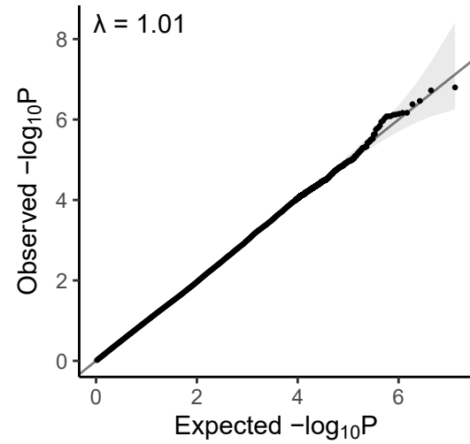
ChrX Gain
