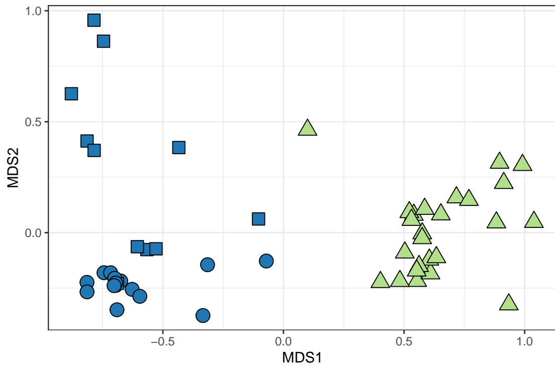
Prokaryote (Stress = 0.06 )
