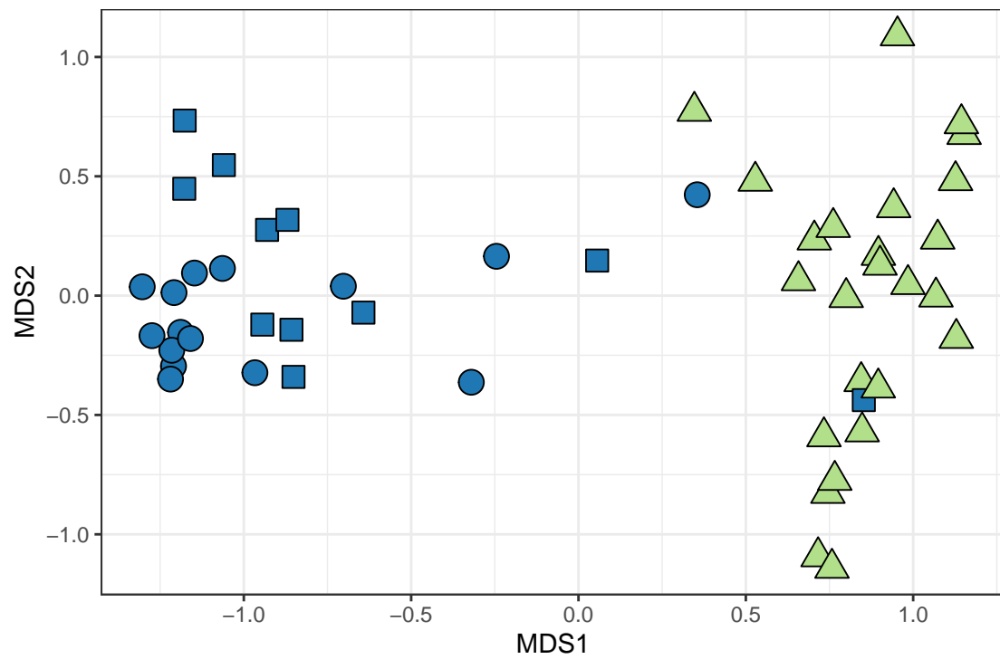
Eukaryote (Stress = 0.08 )
