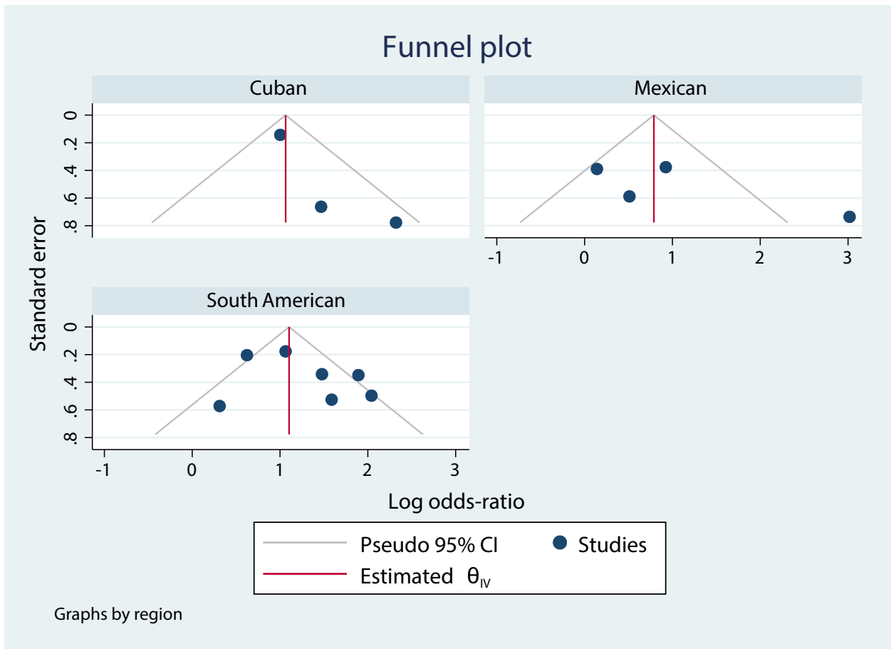
Supplementary Figure 4 ADRD unadjusted funnel
