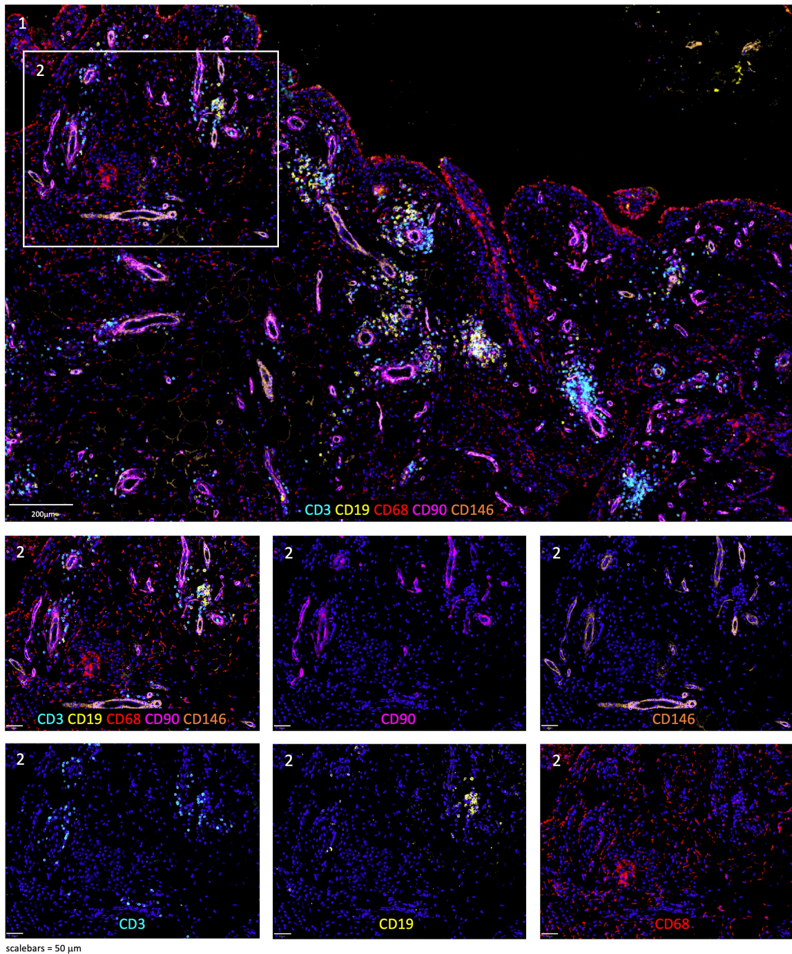
Additional File 12. Immunofluorescence staining of CD90 (pink), CD146 (orange), and immune cell markers CD3 (cyan), CD19 (yellow), and CD68 (red) in advanced OA synovium; DAPI staining was used to visualise nuclei.
