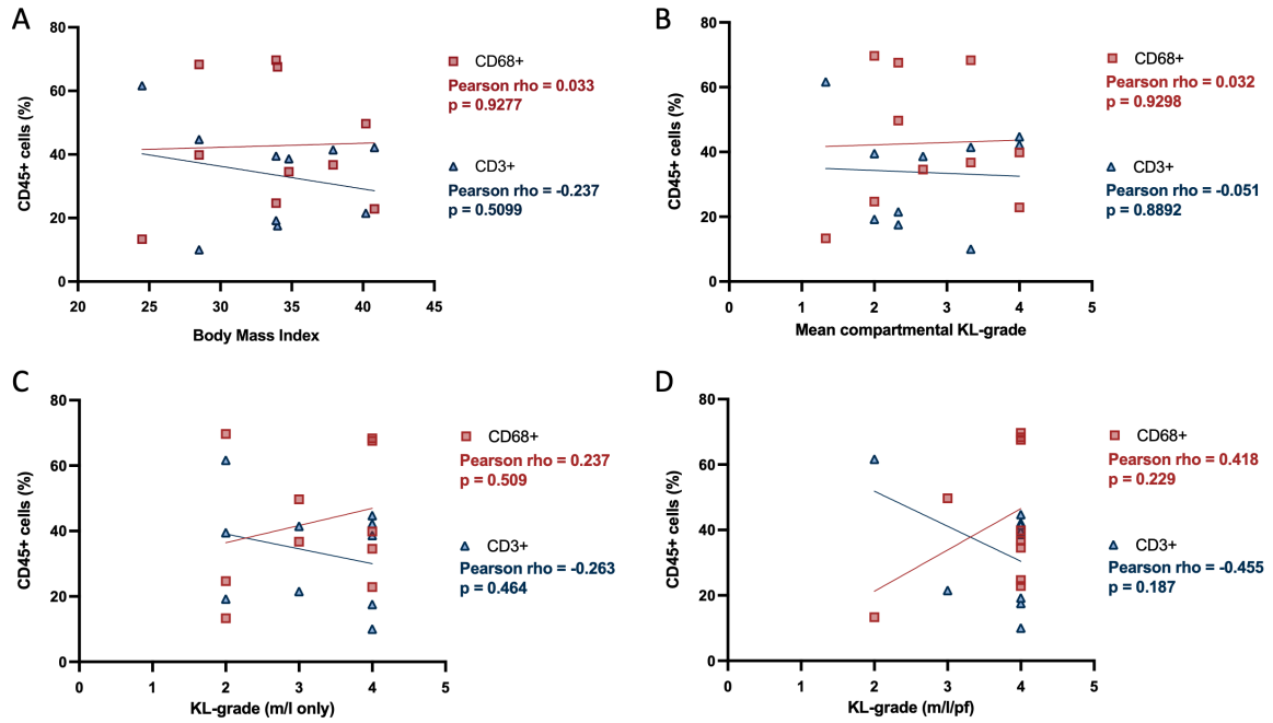
Additional File 6. Relationship between T cells and macrophages (as a percentage of all CD45+ cells) and (A) body mass index (BMI), (B) mean compartmental Kellgren-Lawrence (KL)-grade, (C) KL-grade based on the highest radiographic severity in the medial and lateral compartments only (m/l only), and (D) KL-grade based on the highest radiographic severity in the medial, lateral, and patellofemoral compartments (m/l/pf).
