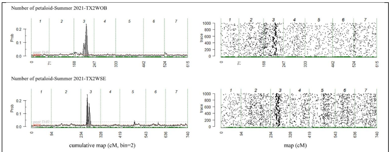
Supplementary Figure 12. Posterior positions (left) and trace samples QTL positions (right) based on an additive model performed using Visual FlexQTL software for number of petaloid phenotyped in Somerville, Texas in summer 2021 for TX2WOB and TX2WSE diploid rose populations.
