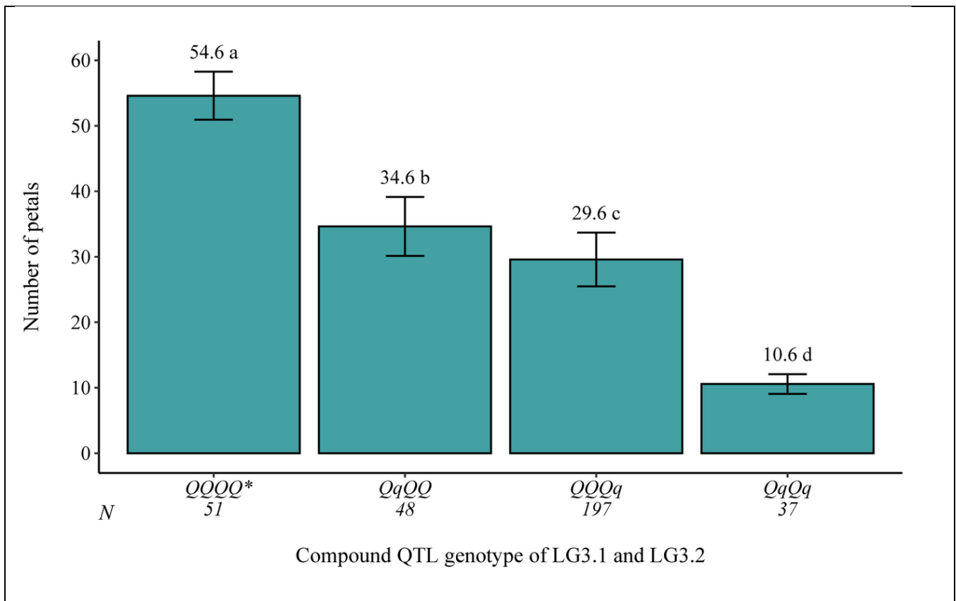
Supplementary Figure 18. Analysis of the compound QTL genotypes from q NP.TX2WOB-LG3.1 and q NP.TX2WOB-LG3.2 on number of petals from all progenies in TX2WOB population. Means not connected by the same letter are significantly different ( P < 0.05 ).
