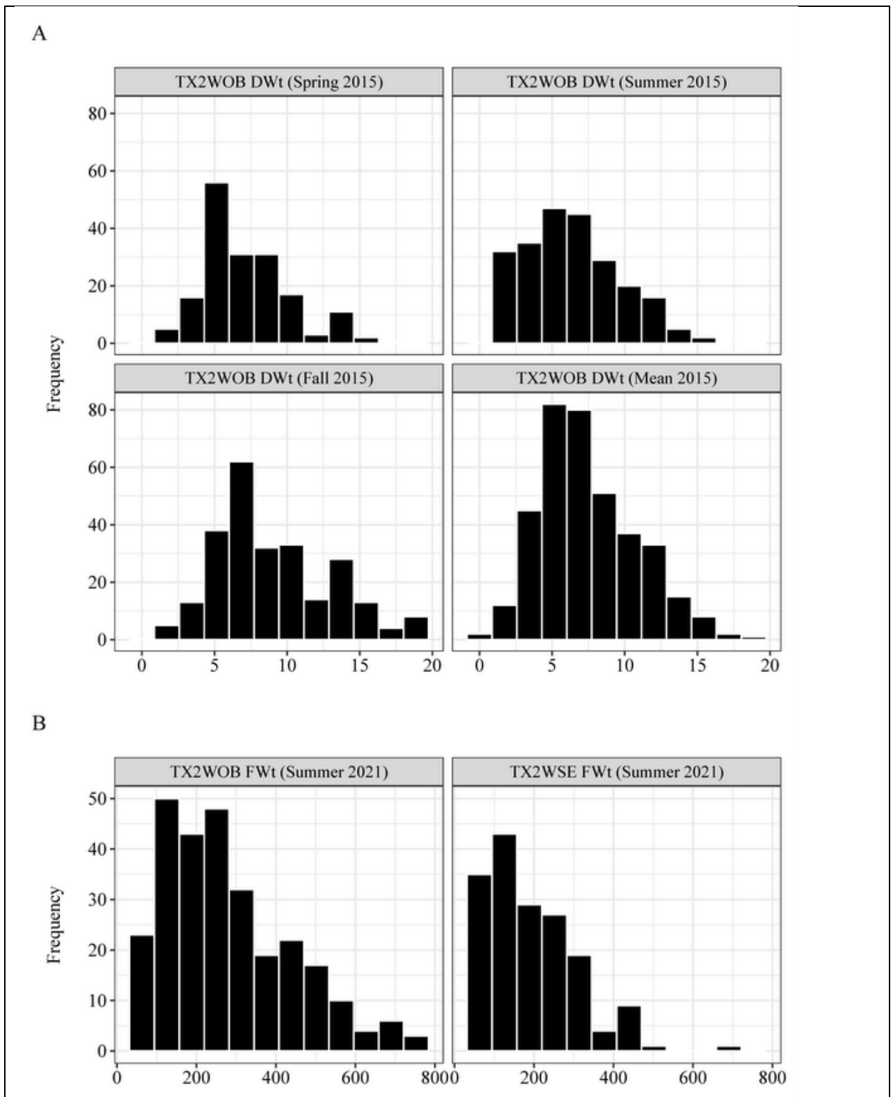
Supplementary Figure 5. Histograms for flower dry weight phenotyped in spring, summer, and fall in 2015 for the TX2WOB diploid rose population (A) and fresh weight in summer 2021 for TX2WOB and TX2WSE (B).
