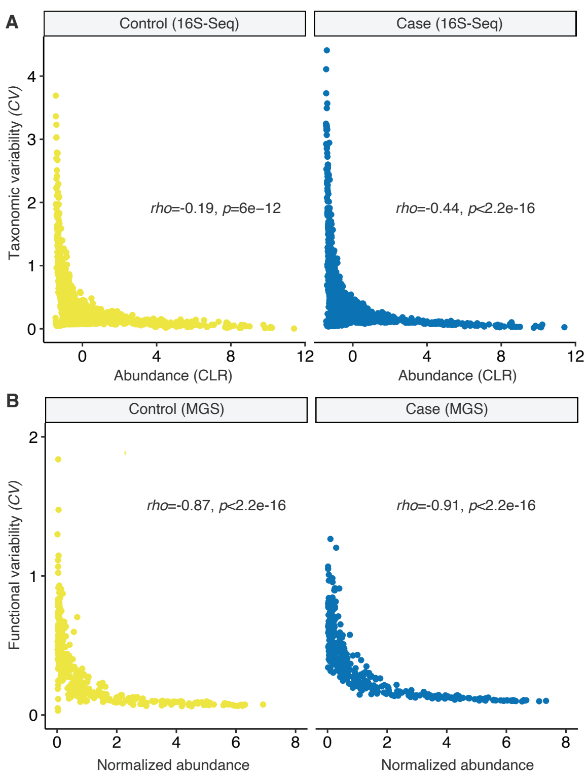
FIG S3 Feature variability negatively correlates with abundance in Cases and Controls. The CV of 16S-Seq ASVs ( A ) or MGS Pathways ( B ) was plotted against the abundance of each and separated between Cases and Controls. A Spearman's correlation coefficient is annotated indicating a negative correlation between CV and feature abundance in all groups. n=18 subjects, 53 samples.
