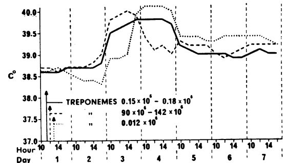
FIG. 1 Mean temperature of thirty rabbits inoculated with 0.15-0.18 \times 10^6 treponemes, twelve rabbits inoculated with 90-142 \times 10^6 , and seven rabbits inoculated with 0.012 \times 10^6 treponemes
