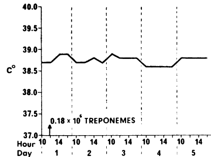
FIG. 6 Effect of re-inoculation with 0.18 \times 10^6 treponemes. Mean temperature of eight rabbits.
