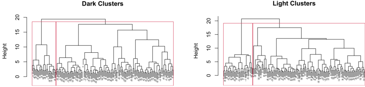
Supplementary Figure 1: Dendrogram representation of agglomerative hierarchical cluster analysis of PACD eyes in the dark (left) and light (right).
