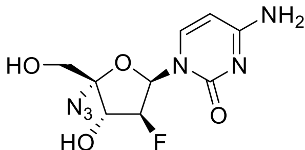
Supplementary Figure S1. Chemical structure of Azvudine.
