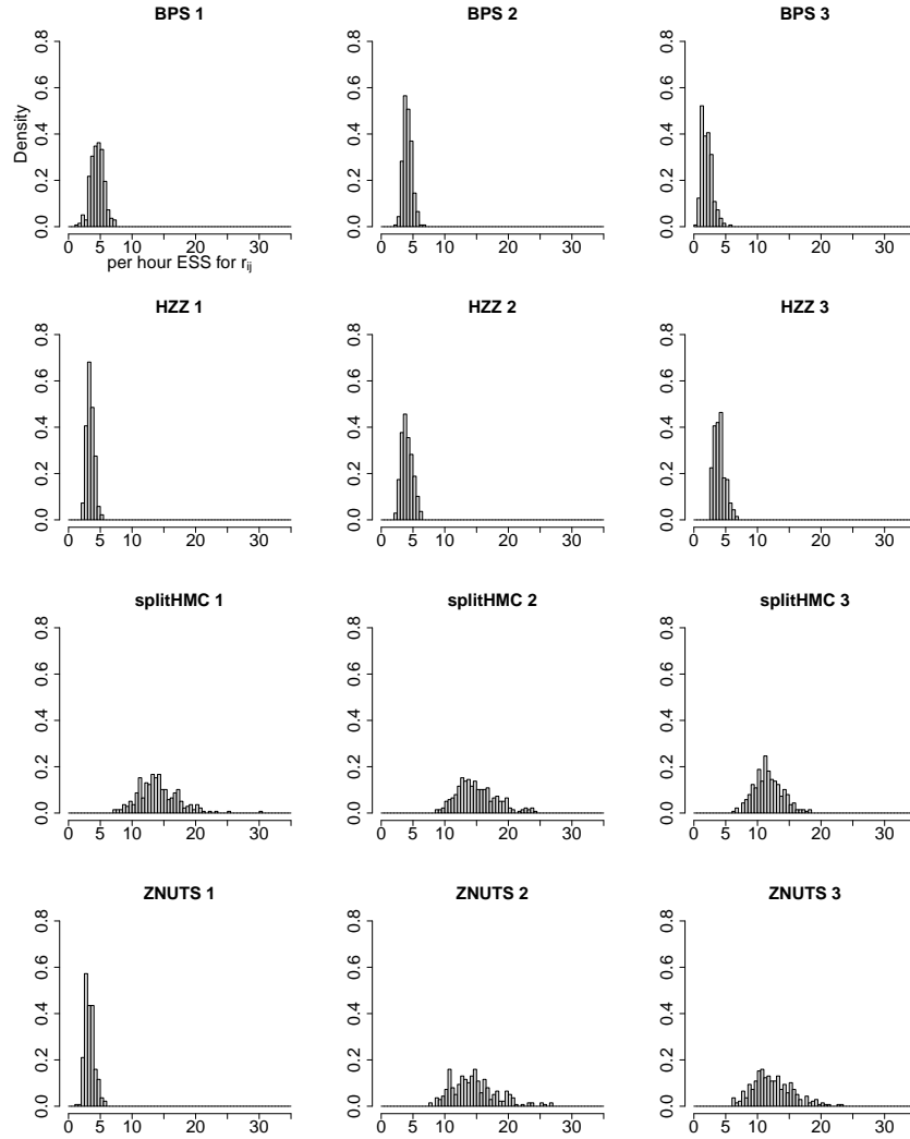
Fig S1: Histograms of per-hour run-time ESS for \mathbf{R} elements, as discussed in Section “Efficiency gain from the new inference scheme”. Each sampling scheme includes three independent repeats (1, 2, 3), and the x-axis and y-axis are consistent across all subfigures.
