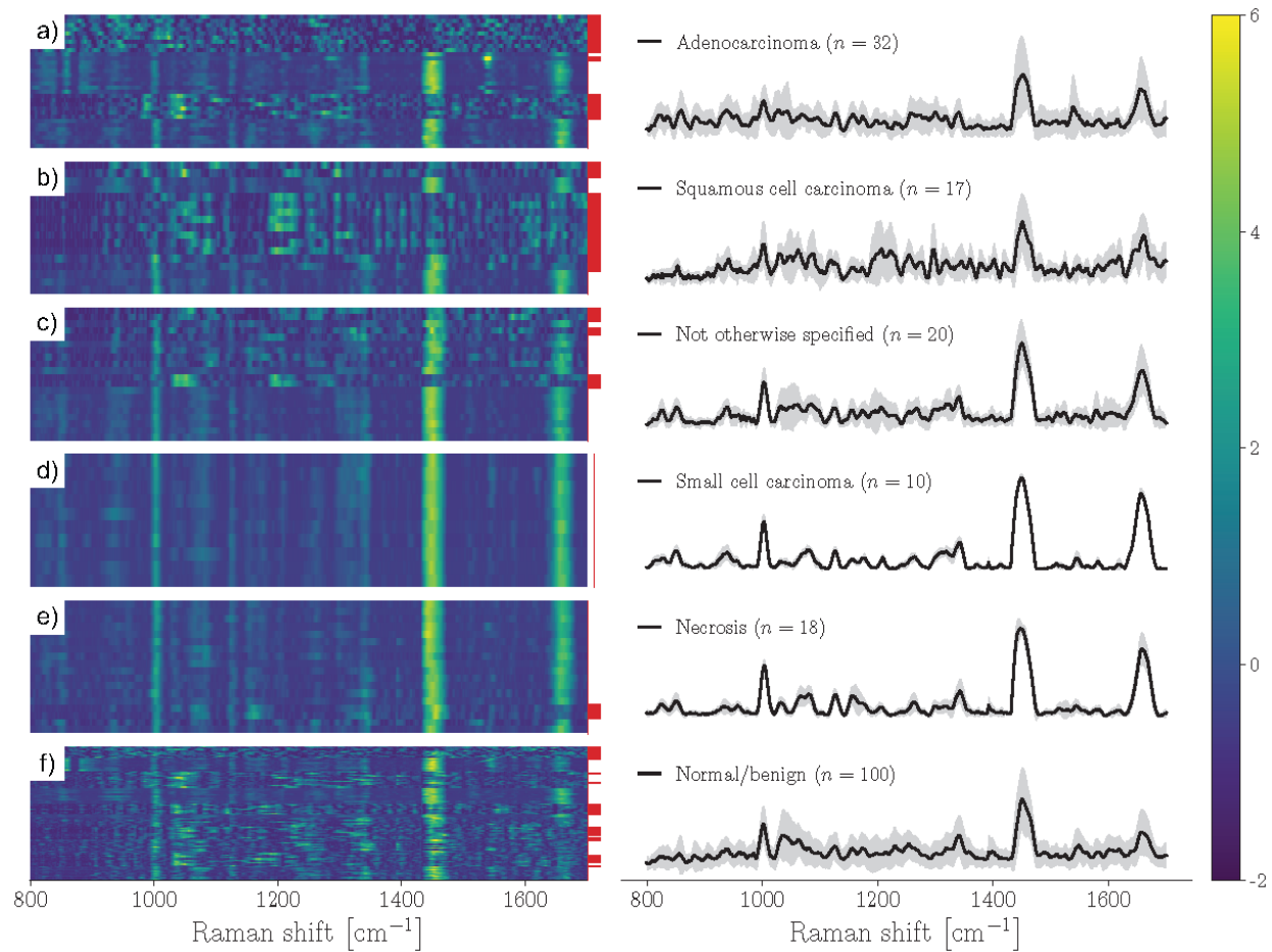
Fig. S1 Raman spectrograms (left) and average Raman spectra with inter-measurements variance (right) for all measurements acquired (no QF cut-off): (a) adenocarcinoma, (b) squamous cell carcinoma, (c) non-small cell cancer of unspecified origin, (d) small cell carcinoma, (e) necrosis, and (f) benign lung tissue. Spectra that were removed to train the models with QF > 0.4 are denoted with a red mark.
