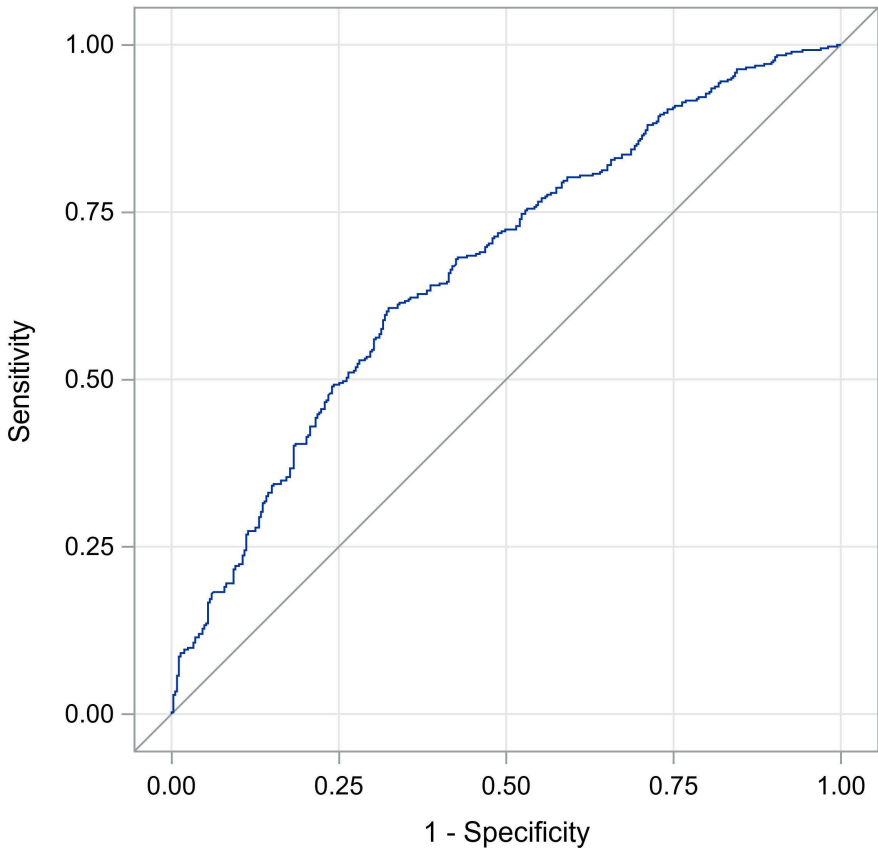
Supplementary Figure 1: ROC Curve for the Model. Abbreviations: ROC – receiver operating characteristic
