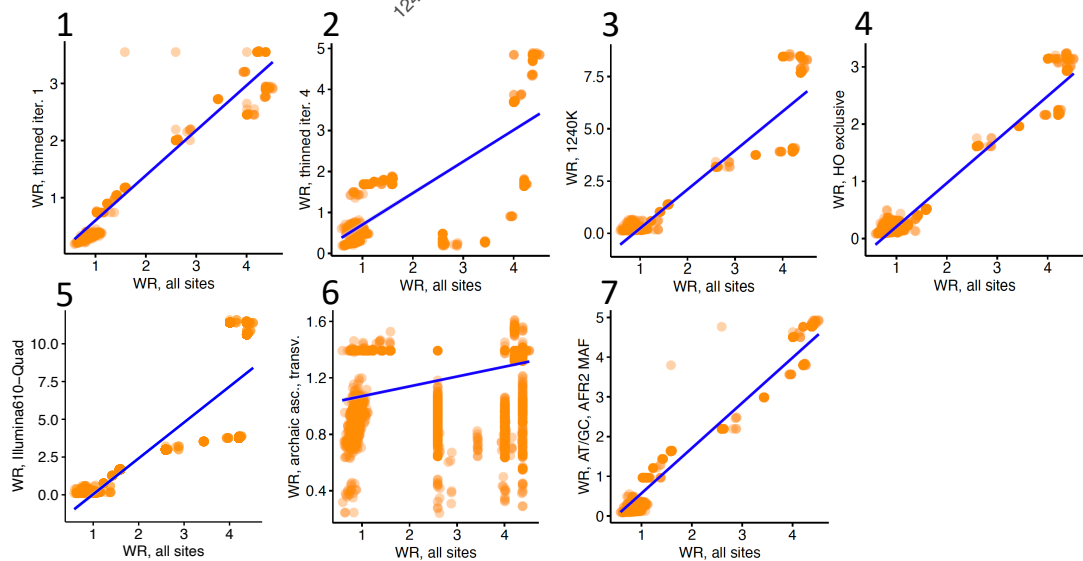
admixture graph WR, 5,000 graphs
