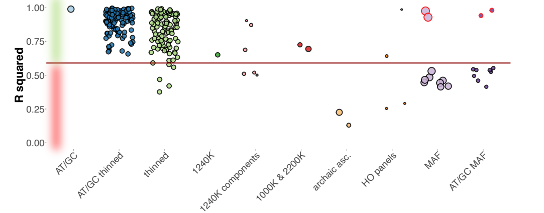
admixture graph WR, 5,000 graphs
