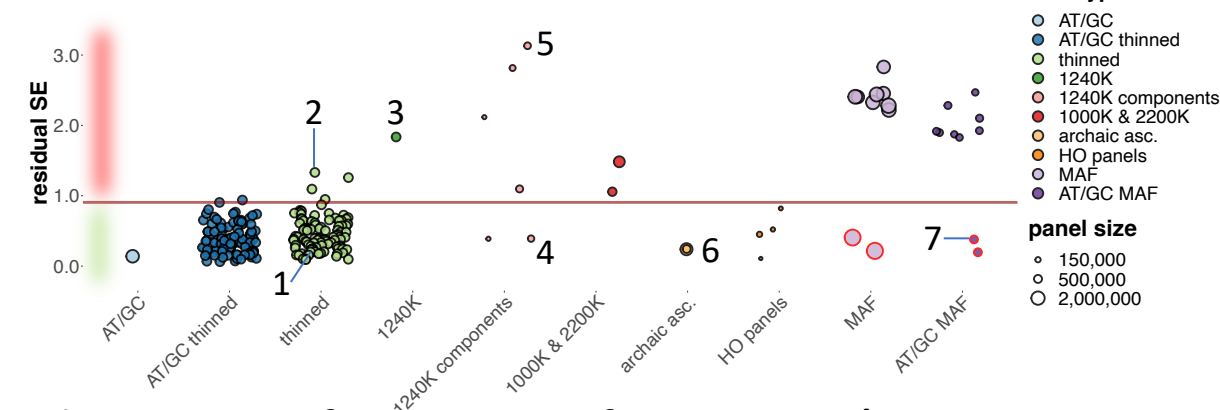
admixture graph WR, 5,000 graphs
