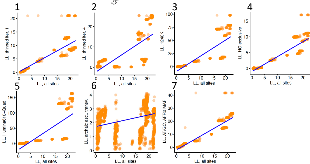
admixture graph LL, 5,000 graphs
