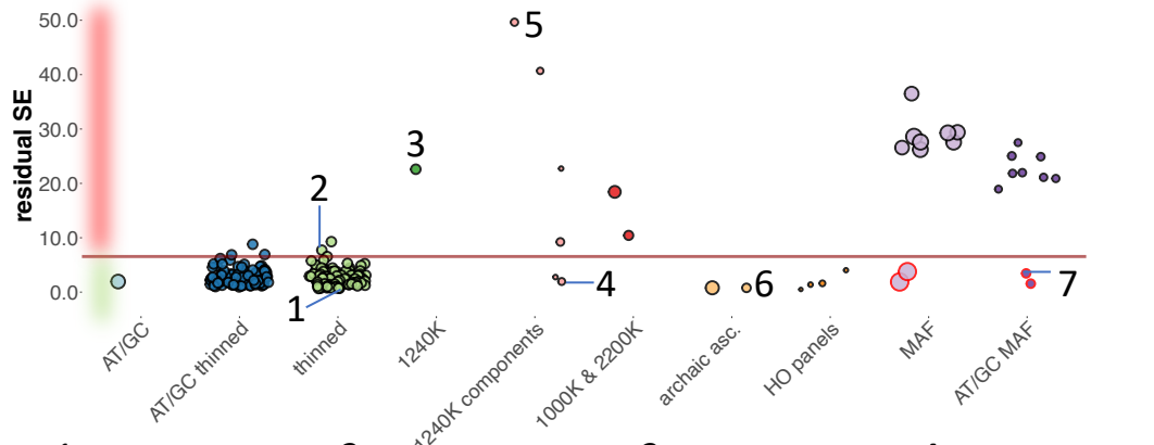
Denisovan, Khomani San, Mbuti, Dinka, Mursi; admixture graph LL, 5,000 graphs
