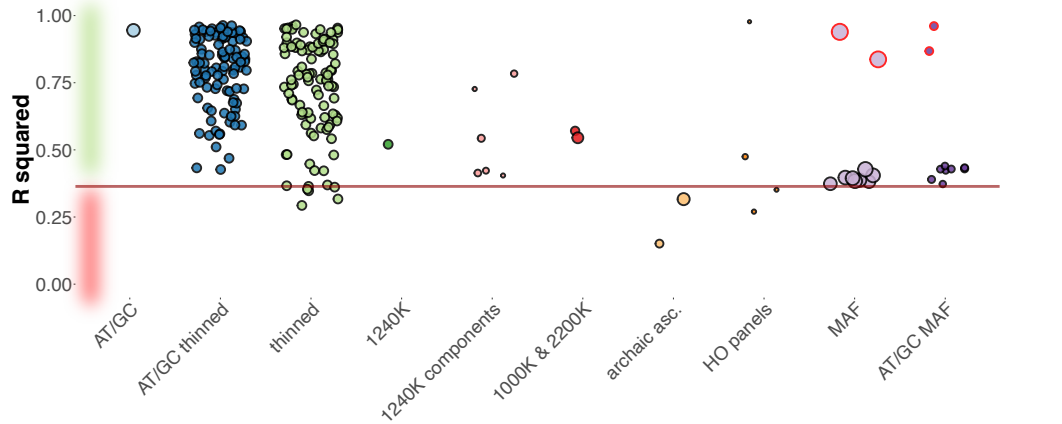
admixture graph LL, 5,000 graphs
