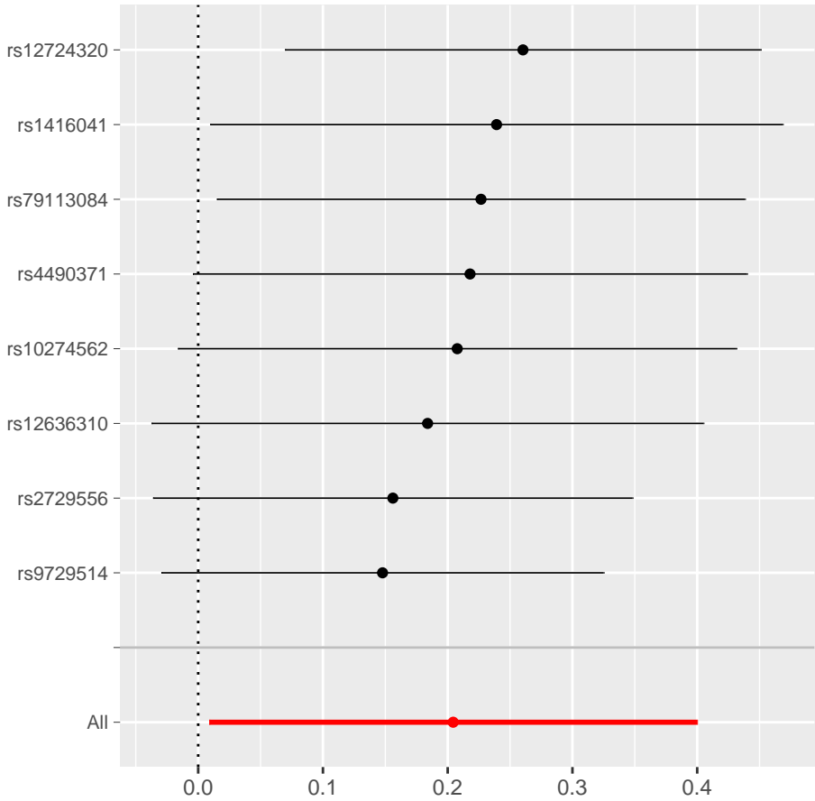
MR leave-one-out sensitivity analysis for
