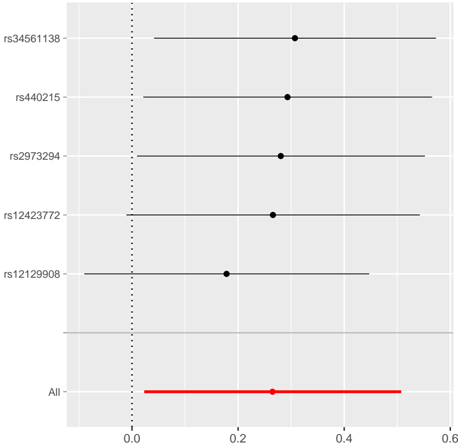
MR leave-one-out sensitivity analysis for
