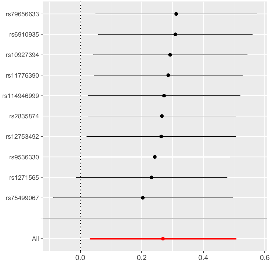
MR leave-one-out sensitivity analysis for 'Age-related macular degeneration (whether dry or wet) || id:ebi-a-GCST90017007' on 'Age-related macular degeneration (whether dry or wet) || id:finn'
