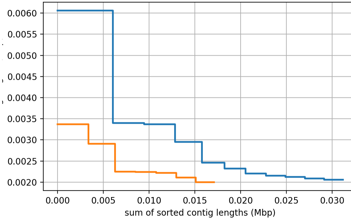
Sorted Contig Lengths (in Mbp)
