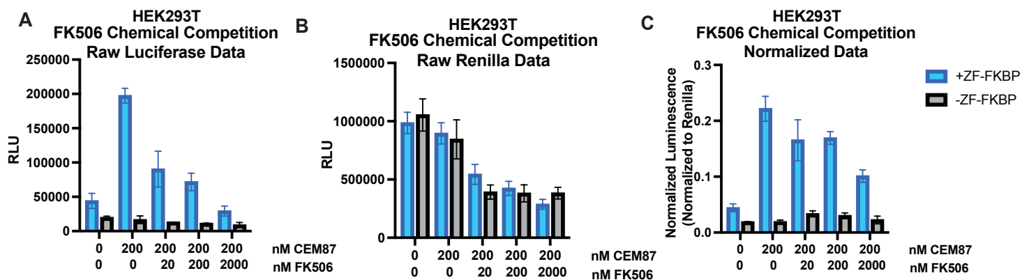
Supplementary Figure 19: Data from infection of 2E+4 vg/cell of AAV2 containing +ZF-FKBP or -ZF-FKBP into HEK293T EF1 \alpha -Renilla cells. Cells were treated with CEM87 and various concentrations of FK506. A. Raw firefly luciferase data, B. Raw renilla luciferase data, and C. Relative firefly luciferase luminescence data normalized to renilla luciferase data.
