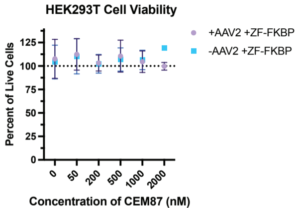
Supplementary Figure 6: Data from HEK293T cells either infected with 2E+4 vg/cell of AAV2 containing +ZF-FKBP or no AAV2 and treated with 0 to 2000 nM of CEM87.
