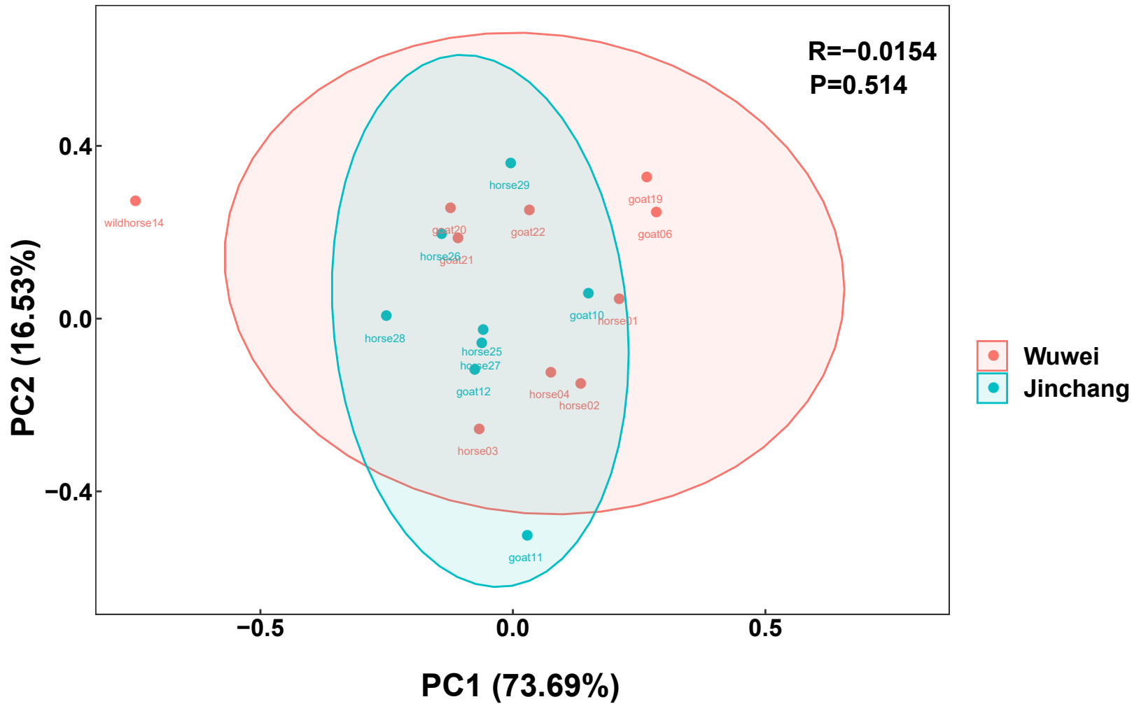
Supplementary Figure 1. PCoA plot of goat and horse of two regions.
