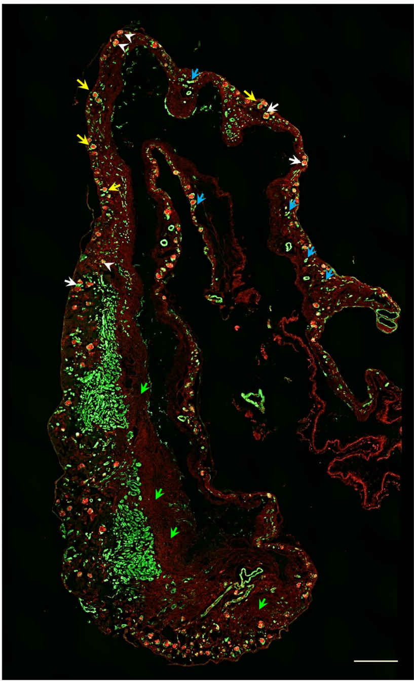
Hydronephrosis Score: 3.5
